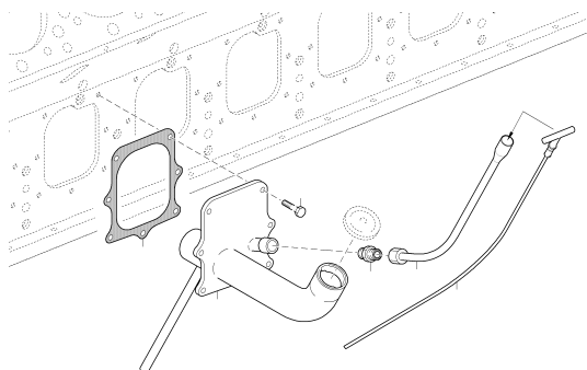
OIL FILLER NECK UPC.06G04 1402
